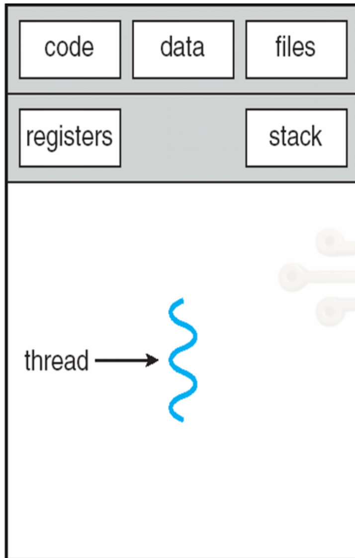
single-threaded process
