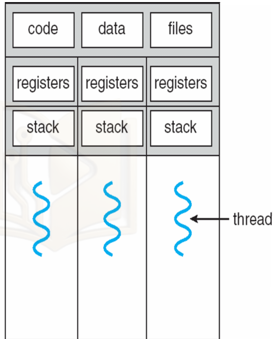
multithreaded process
